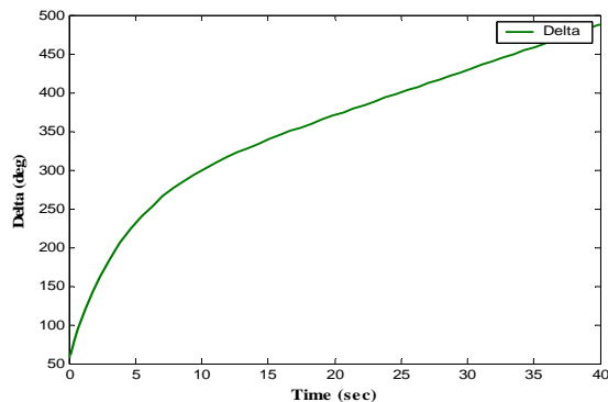
Figure 6. Rotor angle variation with time for X_c = 3
