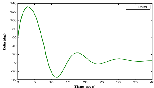
Figure 5. Rotor angle variation with time for X_c = 0.01
