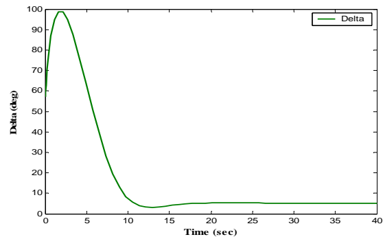
Figure 4. Rotor angle variation with time for k = 30
