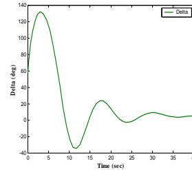
Figure 3 .Rotor angle variation with time for k = 10
