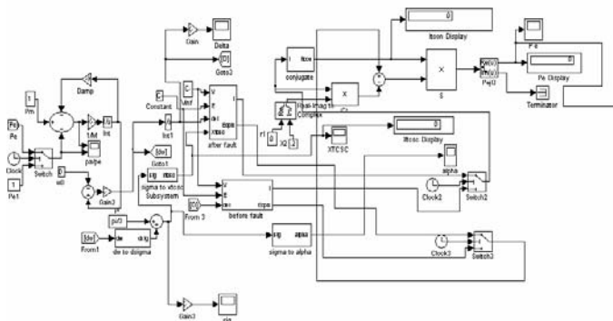
Figure 2. Model of SMIB system using TCSC
